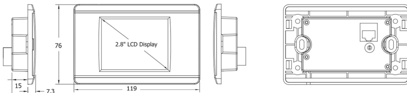
Left View
